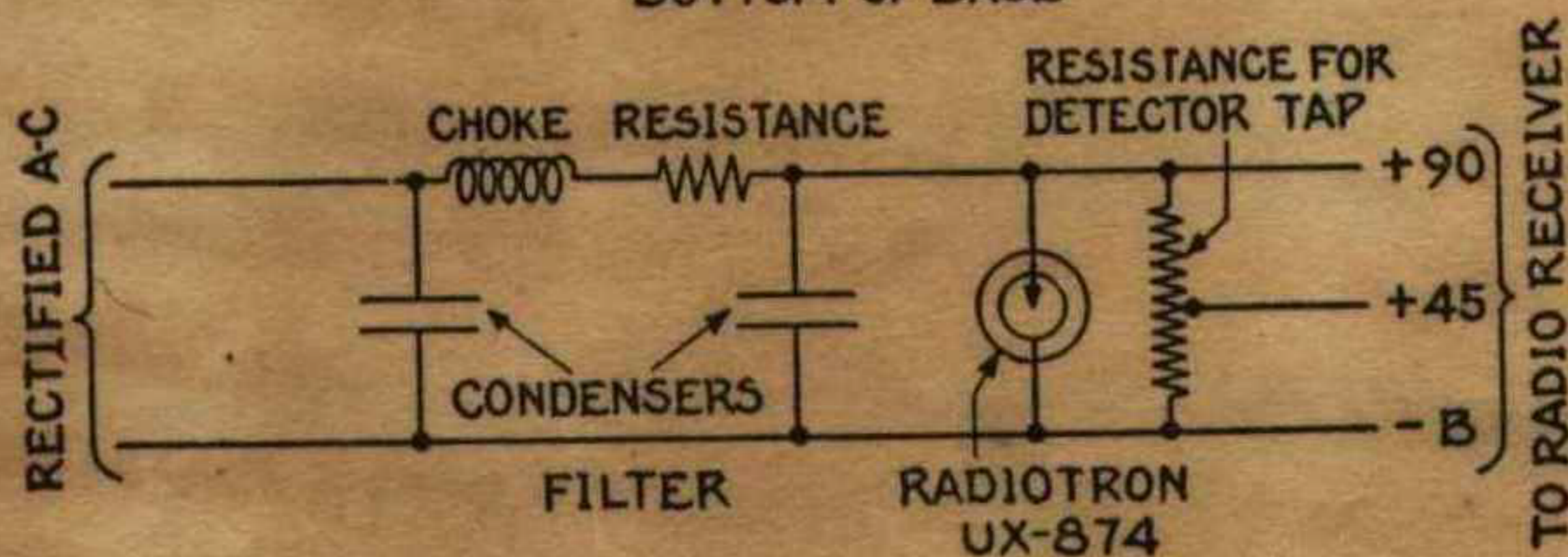
FIG. 2 RADIOTRON UX-874 IN PLATE CURRENT SUPPLY UNIT
